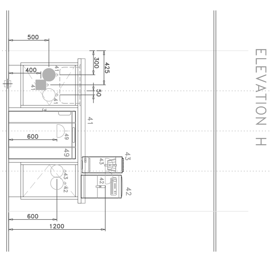
ELEVATION H
